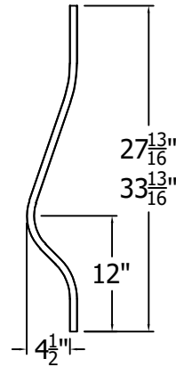
Baluster Side Profile
